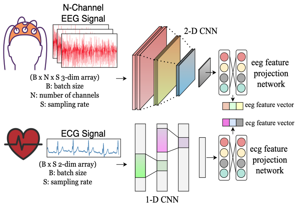
Figure 3. Visualization of representation learning for EEG and ECG signals.
