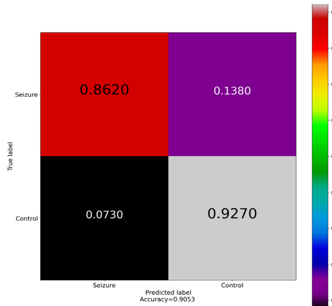
Figure 6. Visualization of Performance of DenseNet-169 Algorithm with Intra Squared Method
